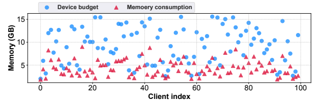
Figure 4: The device memory budget and consumption of running assigned models with memory utilization in targets.
